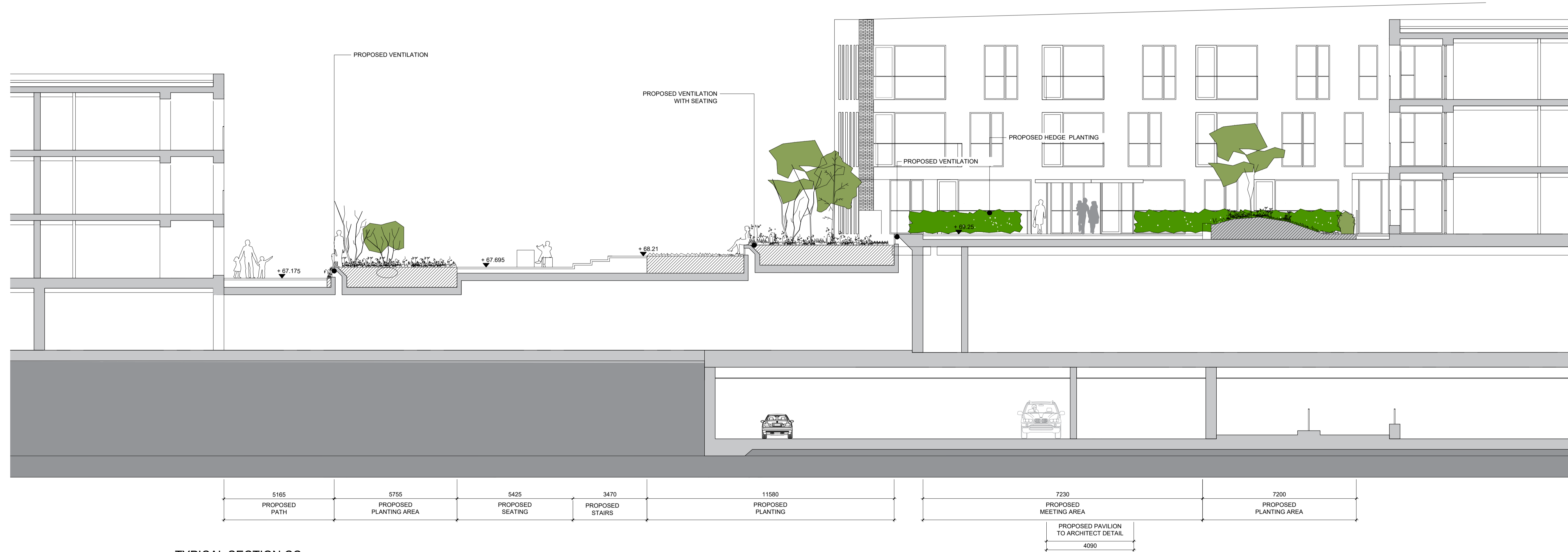
TYPICAL SECTION CC
