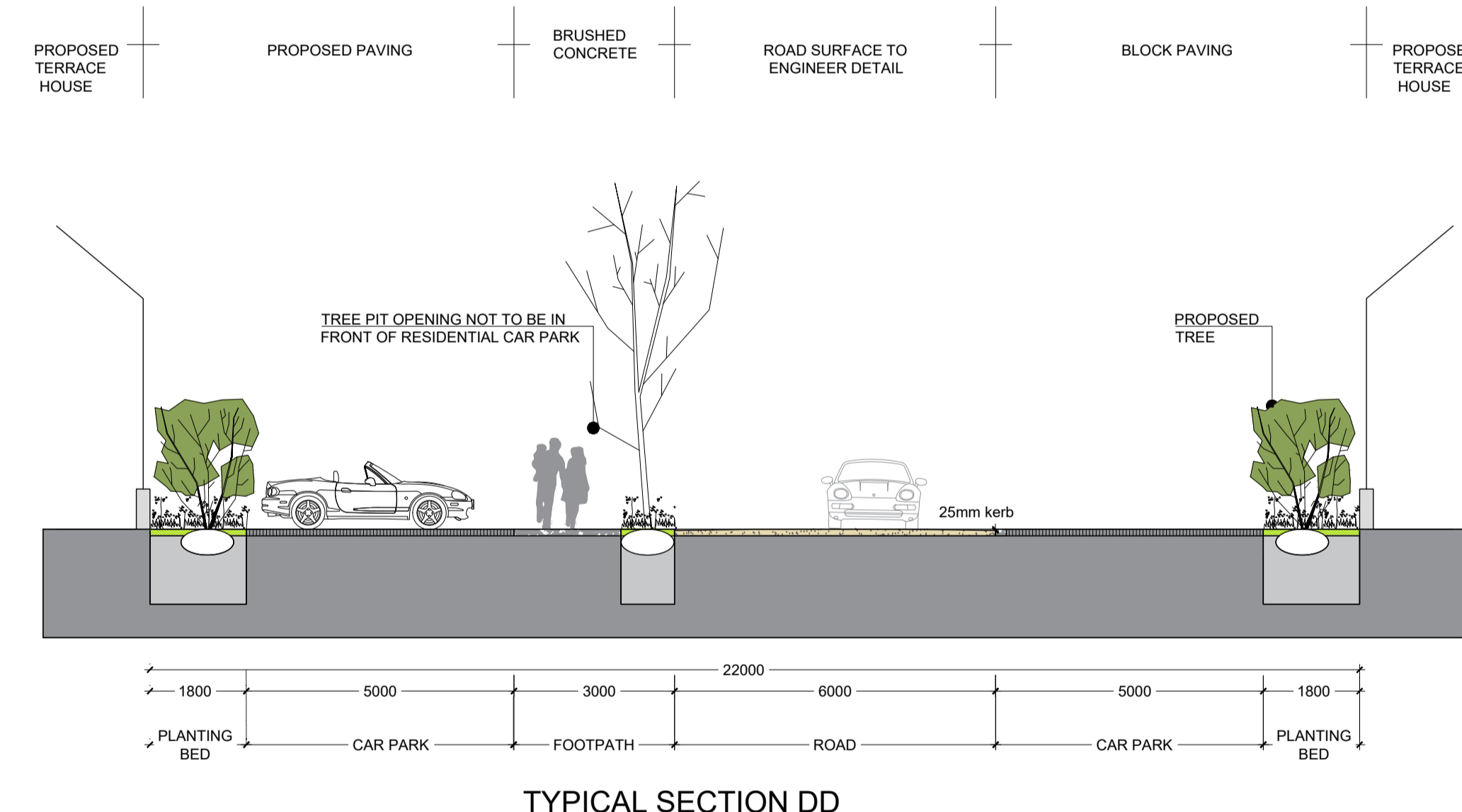
TYPICAL SECTION DD
