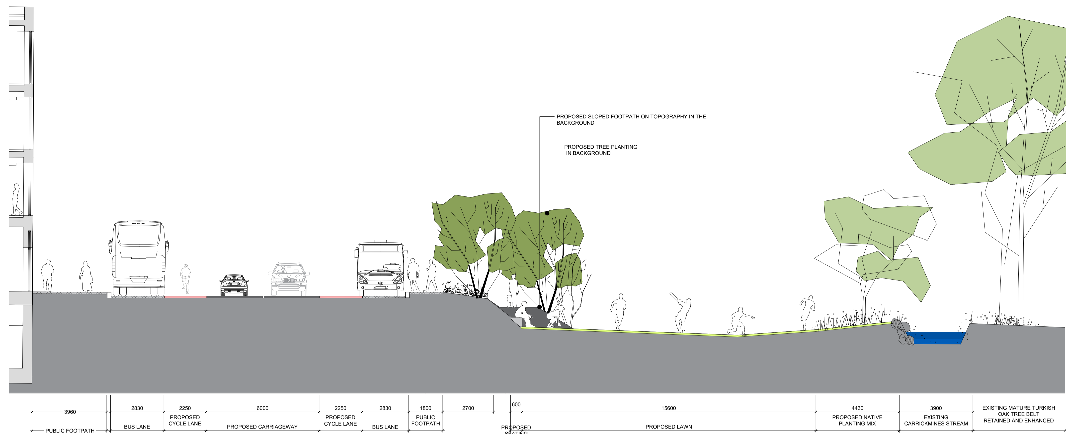
TYPICAL SECTION AA
